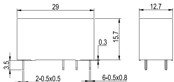
Outline Dimensions
