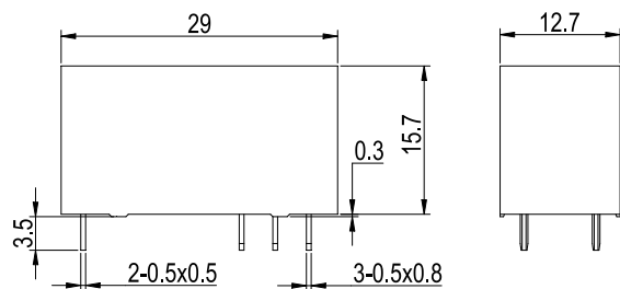
Outline Dimensions
