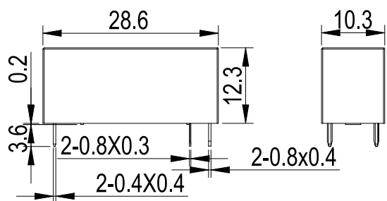
Outline Dimensions
