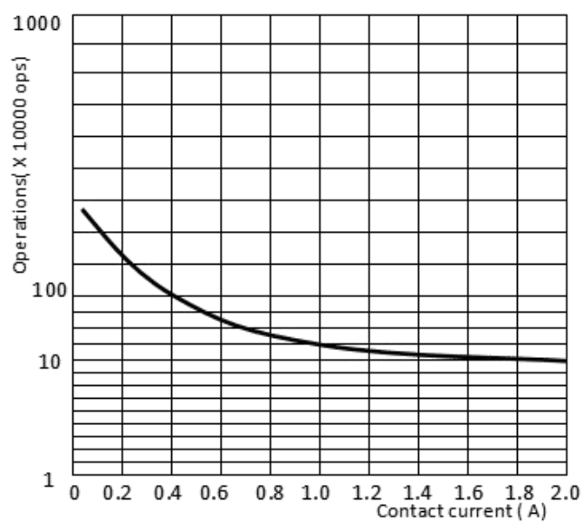
ENDURANCE CURVE
