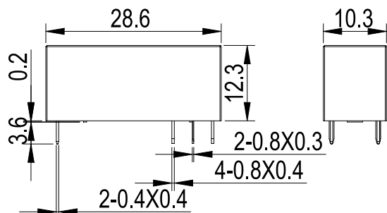
Outline Dimensions
