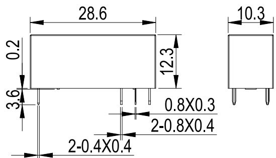
Outline Dimensions
