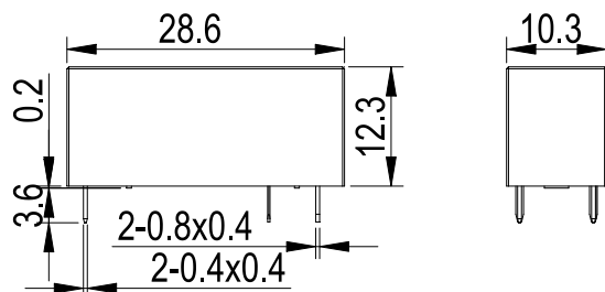
Outline Dimensions
