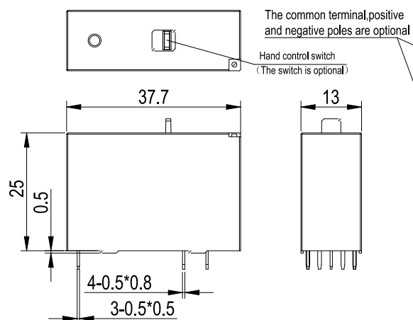
1B Outline Dimensions (Double coils latching)
