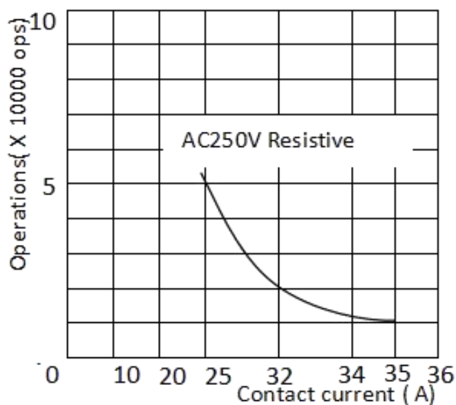
ENDURANCE CURVE
