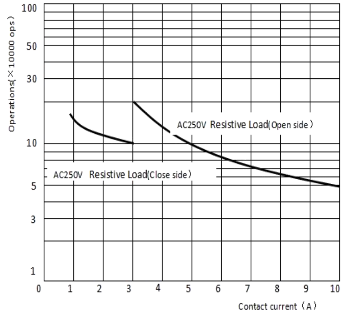
ENDURANCE CURVE
