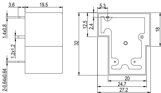
Outline Dimensions
