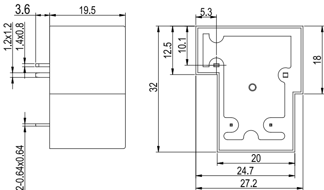
Outline Dimensions
