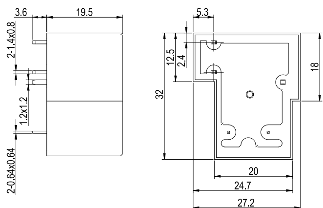
Outline Dimensions
